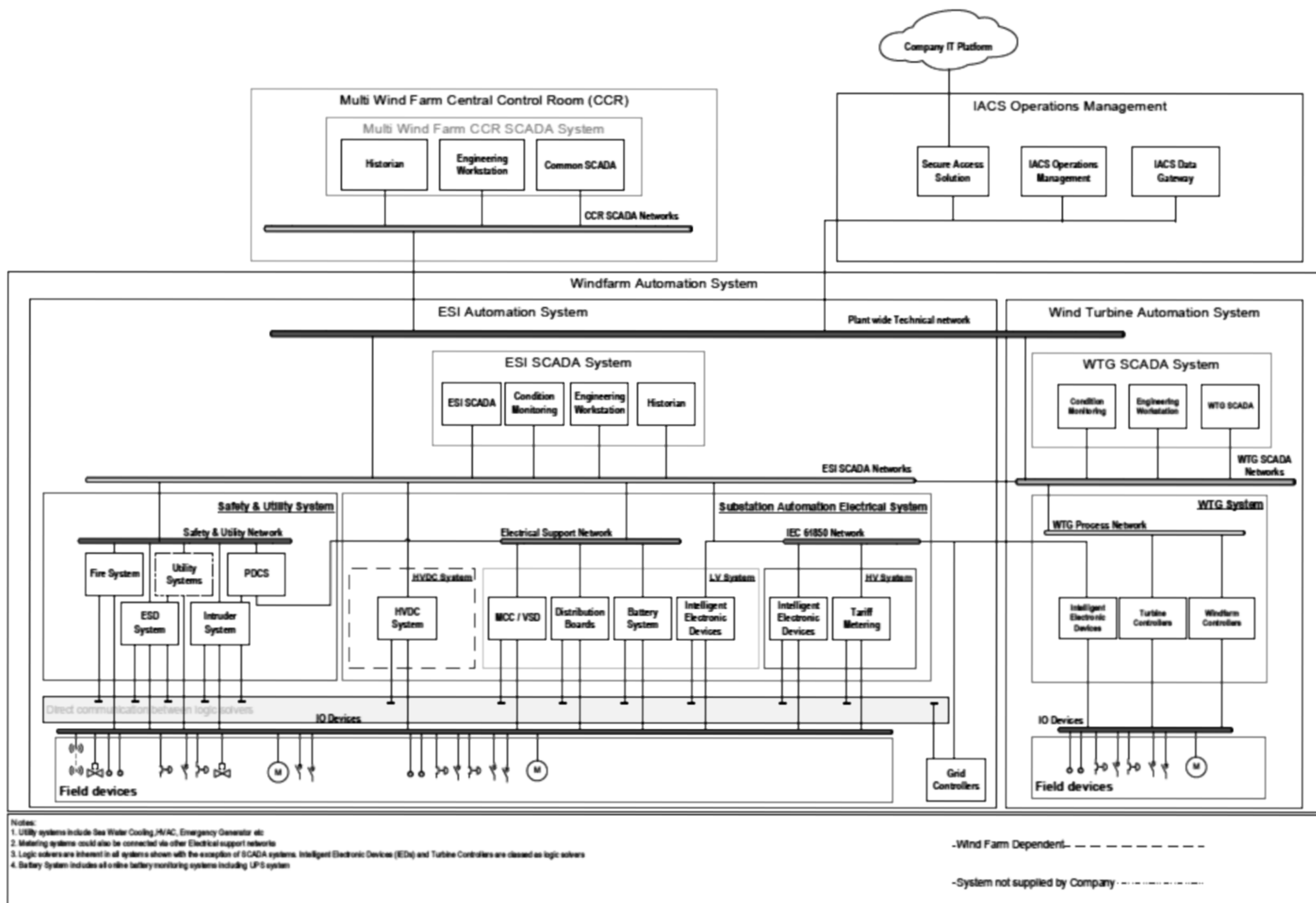
Figure 1 - IACS General Architecture
