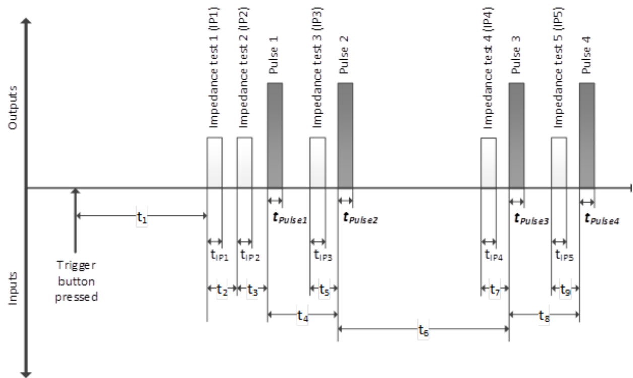
Figure 1 Mechanical Requirement 79 Timing Diagram
